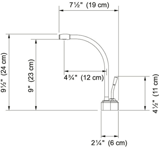
Technical Drawing
