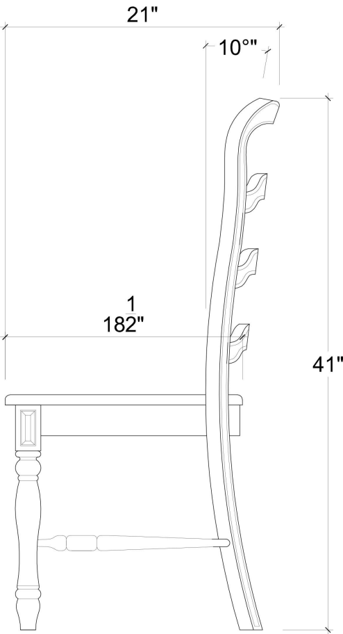
SIDE VIEW
