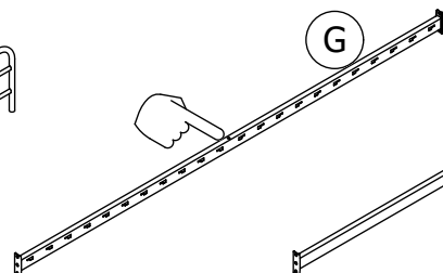
Upper side Rail T922120 X 1
