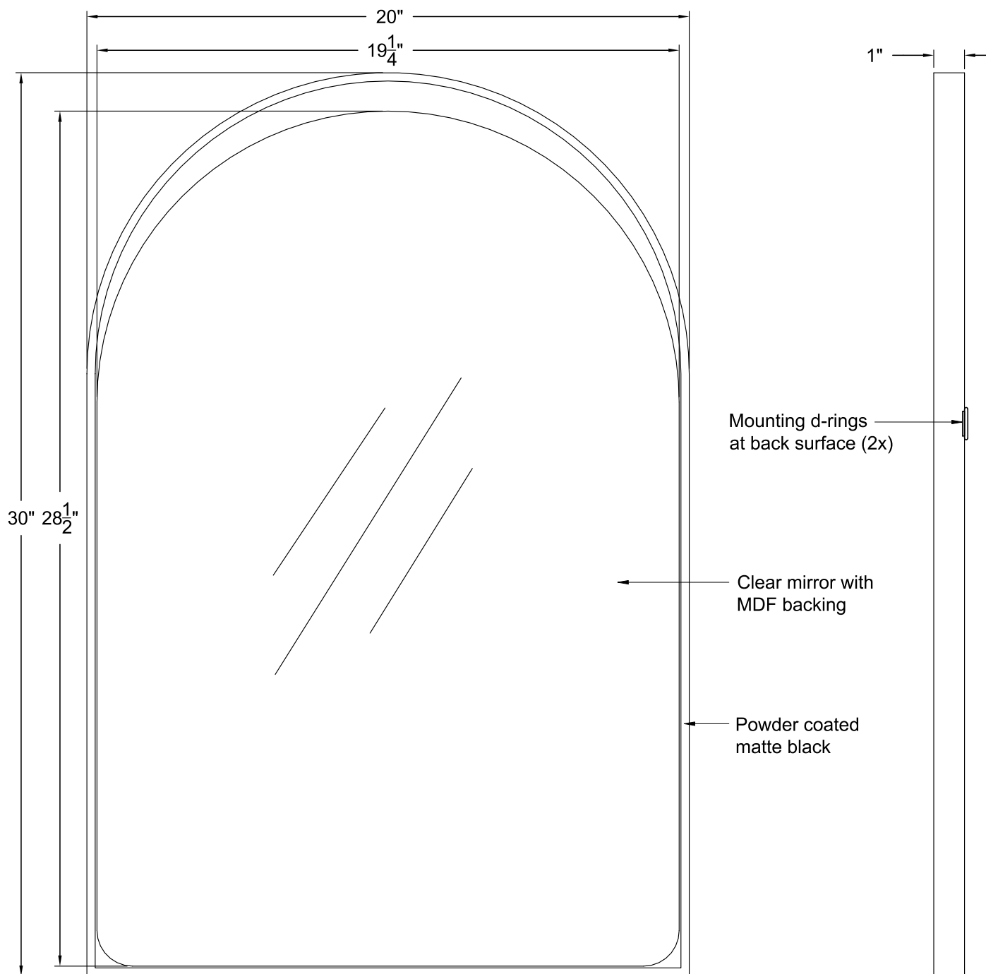
FRONT VIEW
