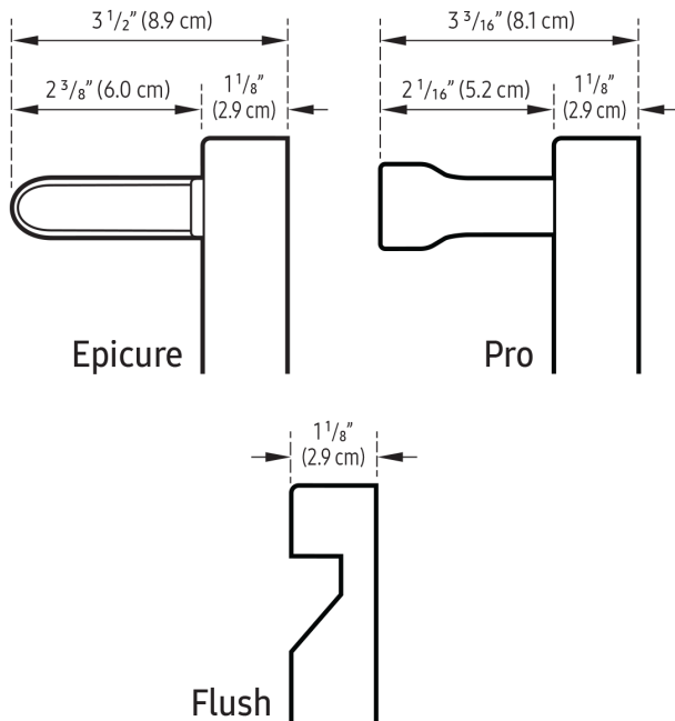
Handle Dimensions
