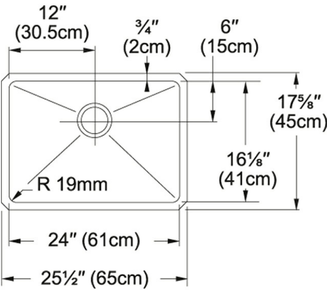
Technical Drawing
