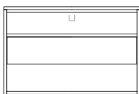
CR9-227 Single Drawer Large Nightstand Case: W36 D18.5 H23.25 (Single Drawer at center; Cord Management opening at top)
