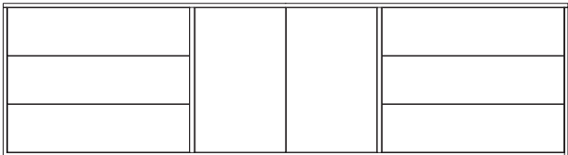
CR9-208-4 Six Drawer Two Center Door Credenza Case: W108 D20.5 H29.25
