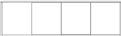
CR9-708 / -408 Four Door Media Console Case: W72 D20.5 H21.25
