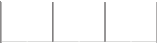
CR9-208-2 Six Door Credenza Case: W108 D20.5 H29.25
