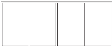
CR9-202 / -203 / -402 / -403 Four Door Credenza Case: W72 D20.5 H29.25 (-203 & -403 One Soft Close Drawer behind each set of doors; -202 & -402 one adjustable shelf behind each set of doors)
