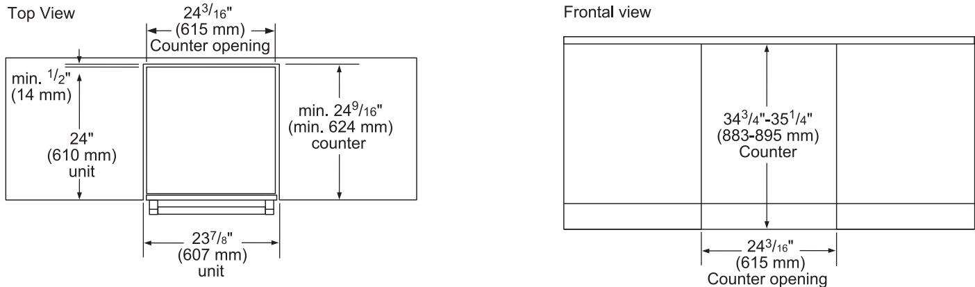
Thermador double drawer under counter top dimension. (Unit door flushed with the cutout)
