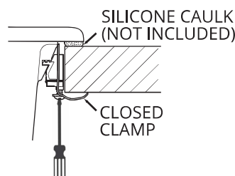
Black/Gray Slotted Screw Clip
