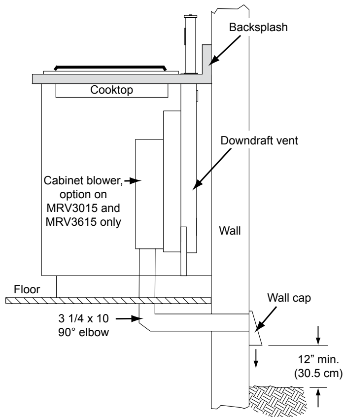
EXAMPLE OF LAYOUT WITH CABINET BLOWER CONFIGURATION, EXHAUST THROUGH WALL
