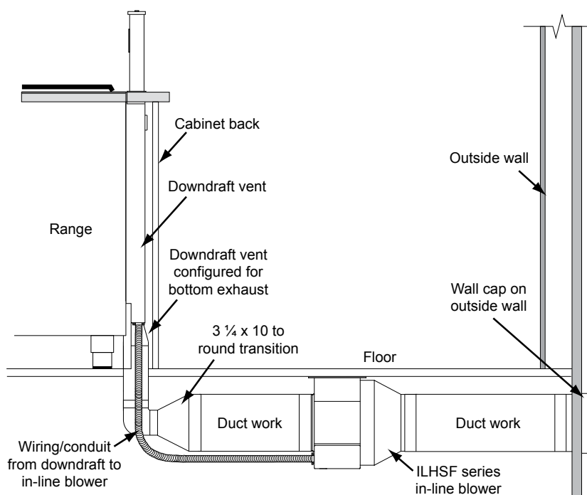
EXAMPLE OF LAYOUT WITH RANGE AND BOTTOM EXHAUST
