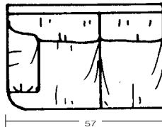
3545-1L LEFT ARM LOVESEAT H36 W57 D39 INSIDE: H17 W48 D22 SEAT H: 20 ARM H: 22
