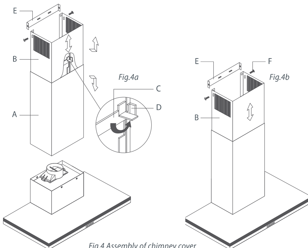
Fig.4 Assembly of chimney cover
