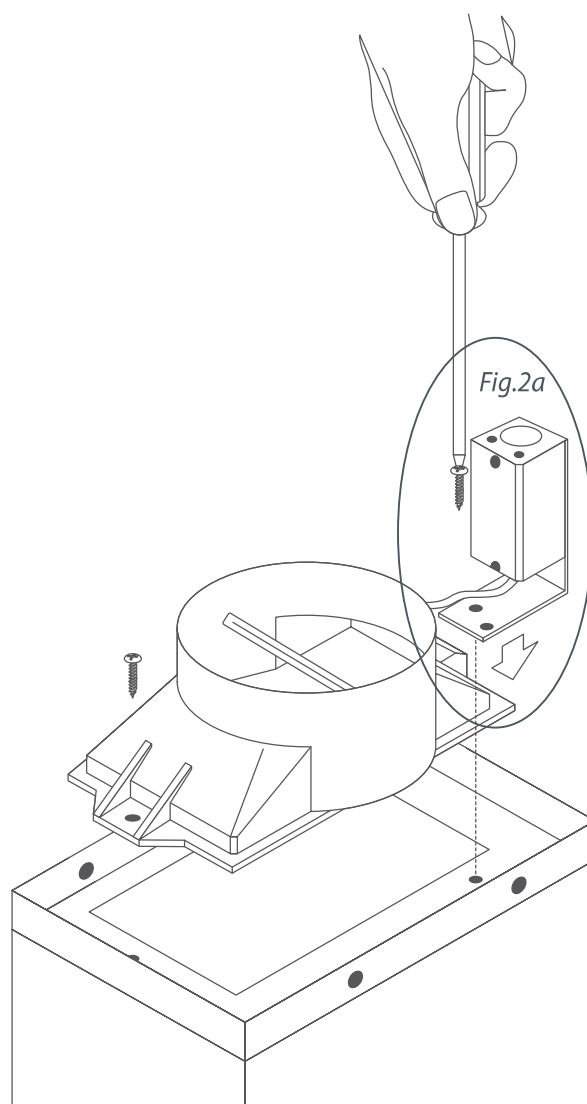
Fig.2 Connect the outlet adapter to the exhaust duct
