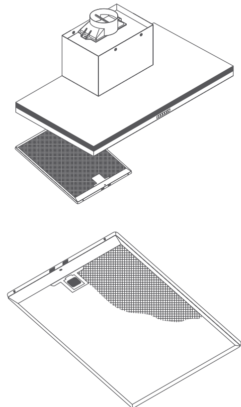
Fig.6 Grease filters
