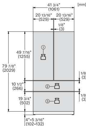
KFMC3858FD, MasterCool III, front view (US)
