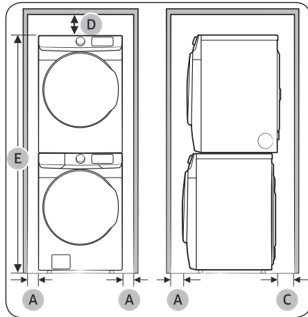
Stacked installation
