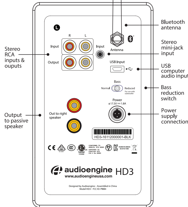
HD3 powered (left) speaker - rear panel
