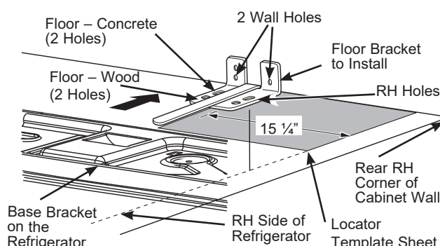
Figure 1 – Installation Overview
