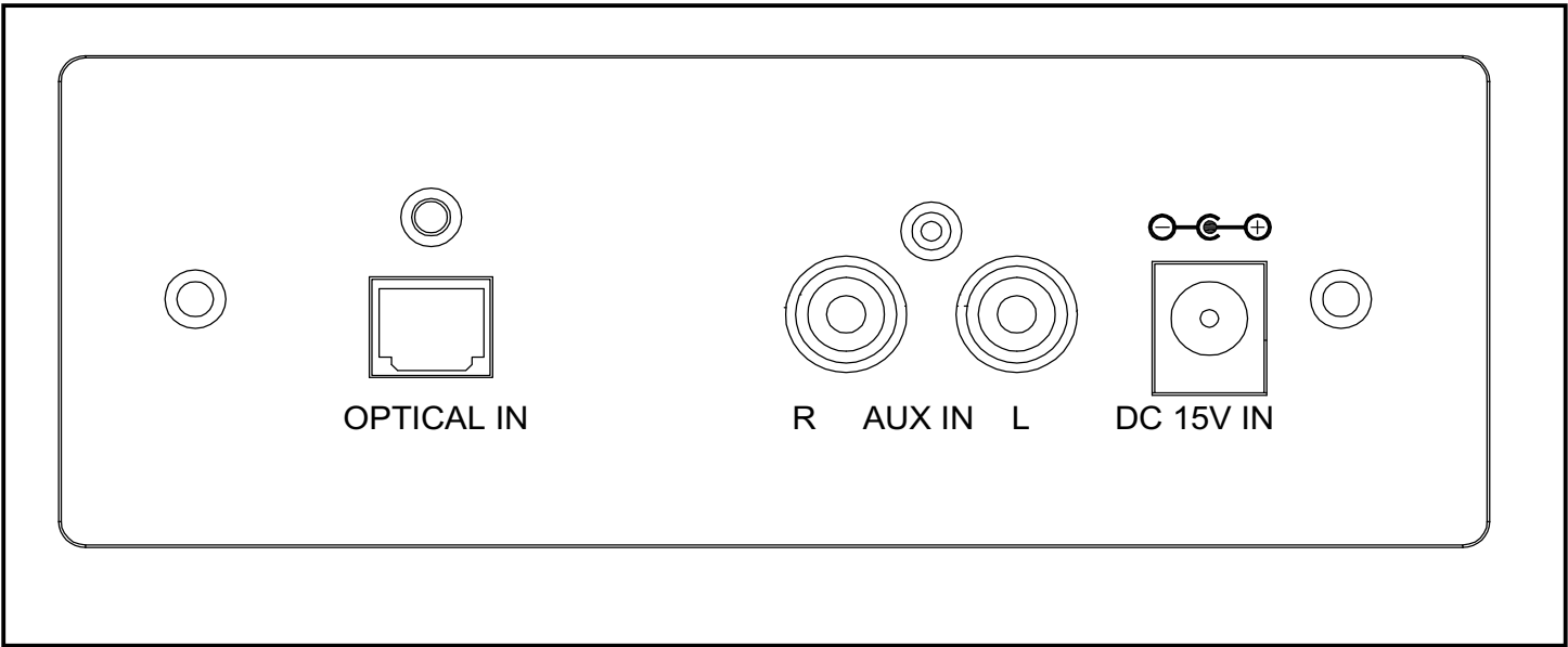
Fig.1 Panel Trasero
