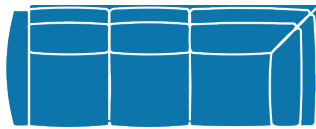
LEFT ARM FACING CORNER SOFA 39 - 70 - 3/3 - LAF OVERALL: H37 W94 D37 INSIDE: W70 D22 SEAT: 20½ ARM: H25½
