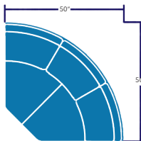
ROUND CHAIR 36 - 3/1 - R OVERALL: H37 W70 D37 INSIDE: W47 D24 SEAT: H20½
