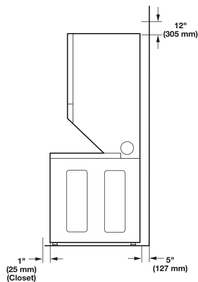
Front/Back/Top Clearances
