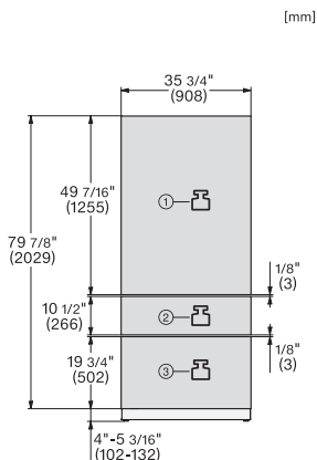
KFMC3846R, KFMC3846L, MasterCool III, front view, installation (US)
