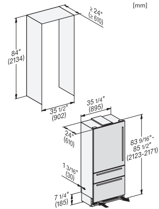
KFMC3846R, KFMC3846L, MasterCool III, PACS, with stainless steel front, integration (US)
