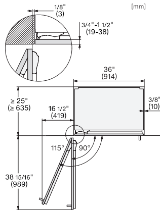
KFMC3846R, KFMC3846L, MasterCool III, panel ready, top view (US)
