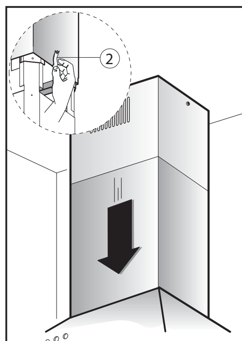
Fig.6: Remove adhesive tape 2 and rest the lower chimney piece above the cooker hood.
