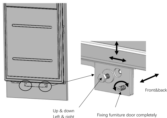
Fixing furniture door completely
