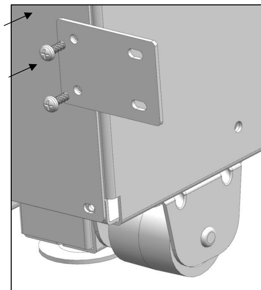
Connecting bracket
