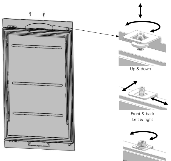
Fixing furniture door completely
