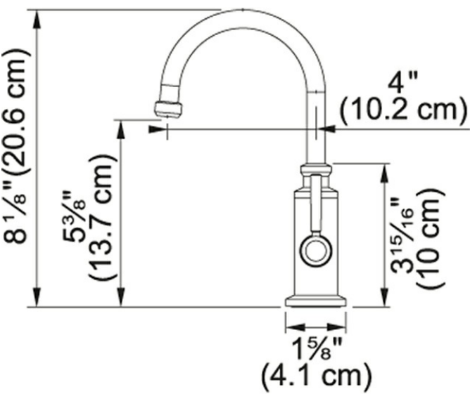
Technical Drawing
