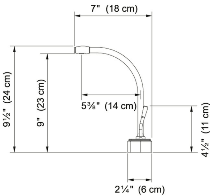
Technical Drawing
