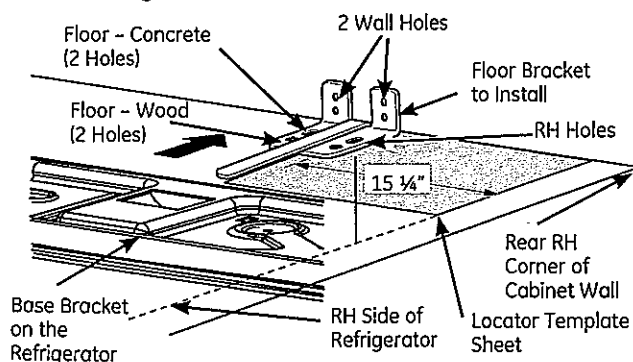
Figure 1 - Installation Overview
