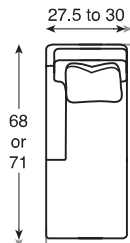
LTD3000-81 LAF Chaise W27.5-30 D68/71 H35.5 1 TP (20x20) T-Cushion only
