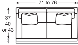
LTD3000-3 Apartment Sofa W71-76 D37/40/43 H35.5 2 TPs (20x20)
