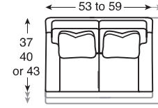
LTD3000-4 Love Seat W53-59 D37/40/43 H35.5 2 TPs (20x20)
