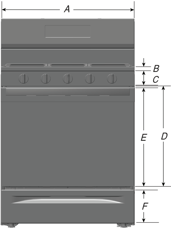
VISTA FRONTAL
