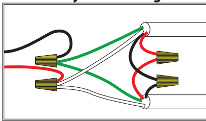
Right Channel Daisy-chain wiring.
