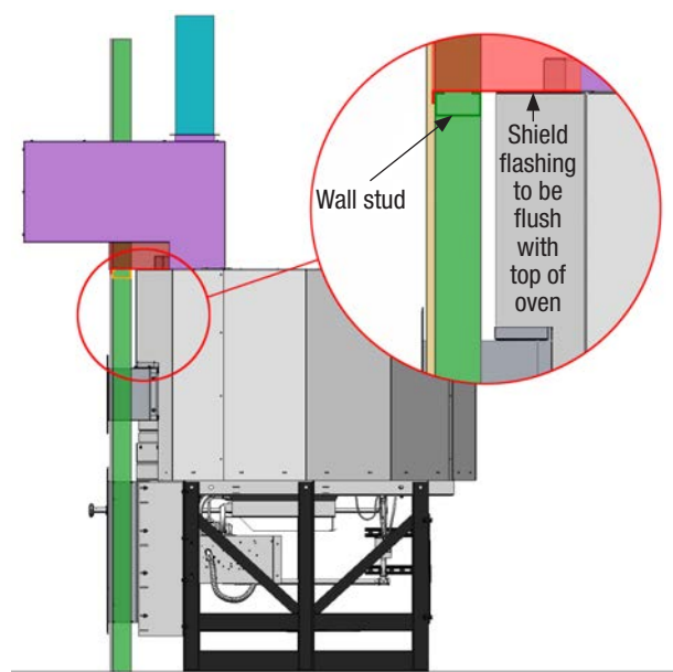
Acceptable venting
