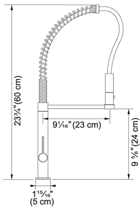
Technical Drawing
