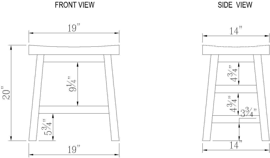
AMBA2020 POMONA STANDARD HEIGHT STOOL
