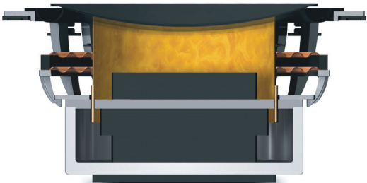
Conventional driver traps air inside
