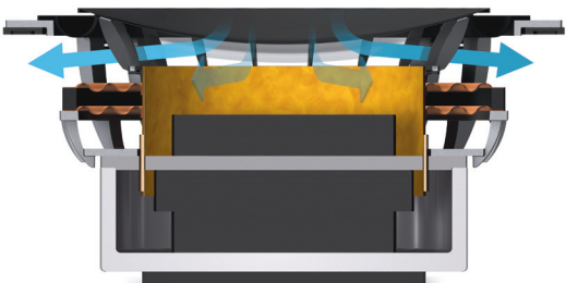
Blade driver with a vented coupler
