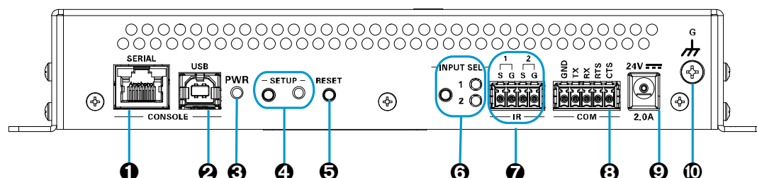
DM-NVX-350 and DM-NVX-351 Front Panel
