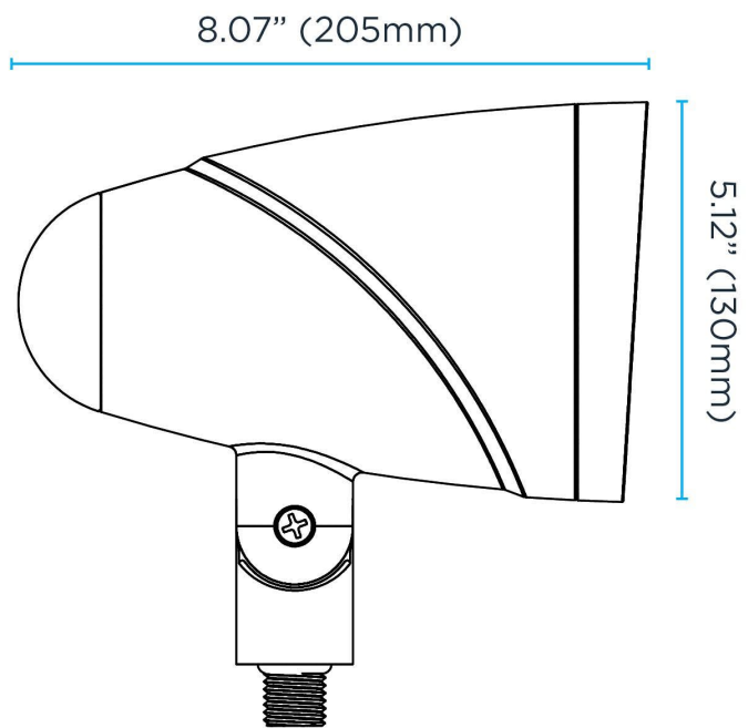
SLS LS4T Speaker Side View
