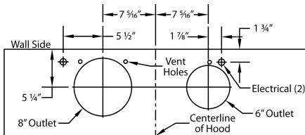
900 CFM B200 Dual &amp; B100 Single Blower (Top View)
