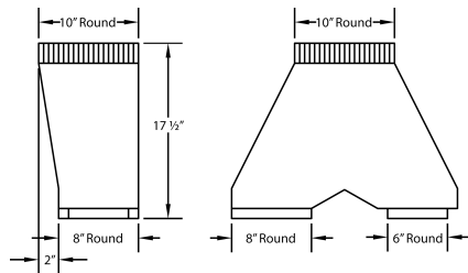
900 CFM B200 Dual &amp; B100 Single Blower (Top View)
