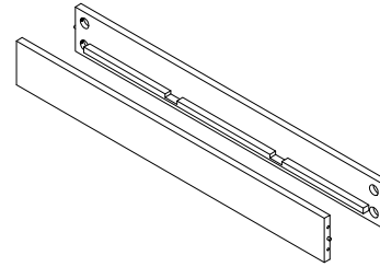
P3 Side rail (x 1)
