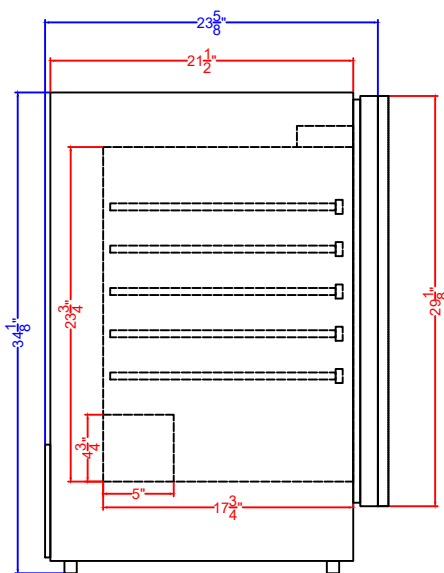
Panel Dimensions See manual for exact installation instructions
