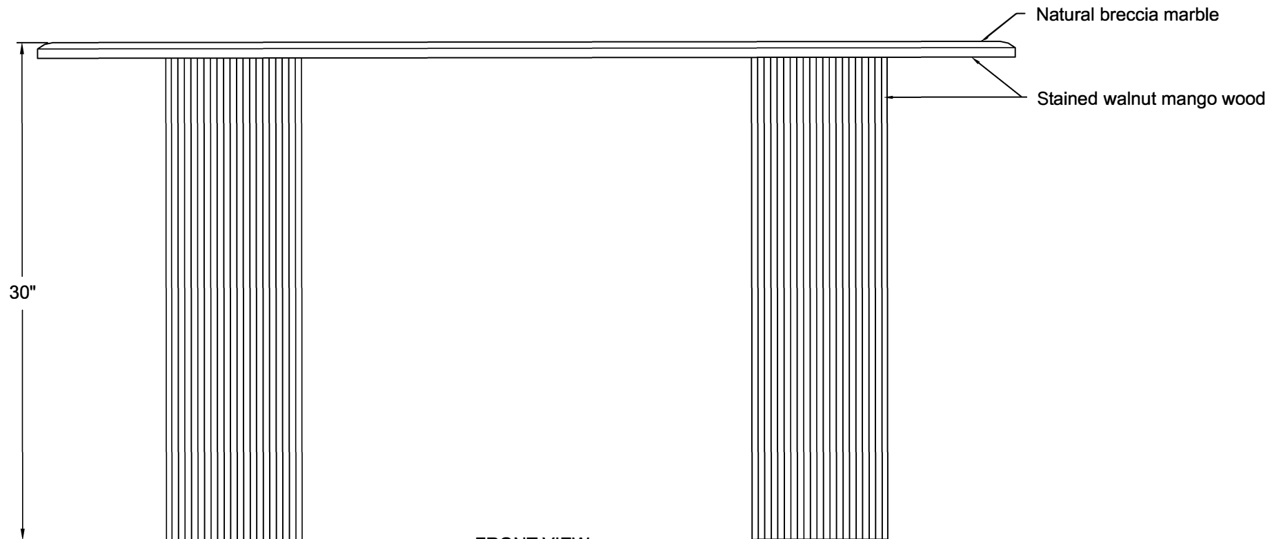
FRONT VIEW
