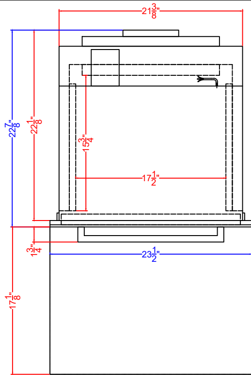
Top View
