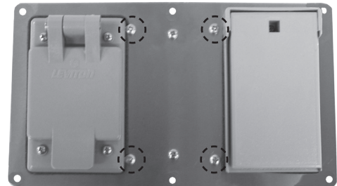
Fig. 41-3 Remove 4 small screws
