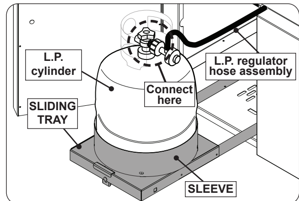
Fig. 7-2 Place and connect cylinder
