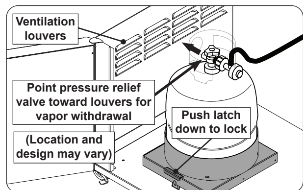
Fig. 7-3 Position cylinder and secure tray
