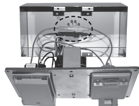
Fig. 41-4 Carefully open box and replace fuse (red wire)
