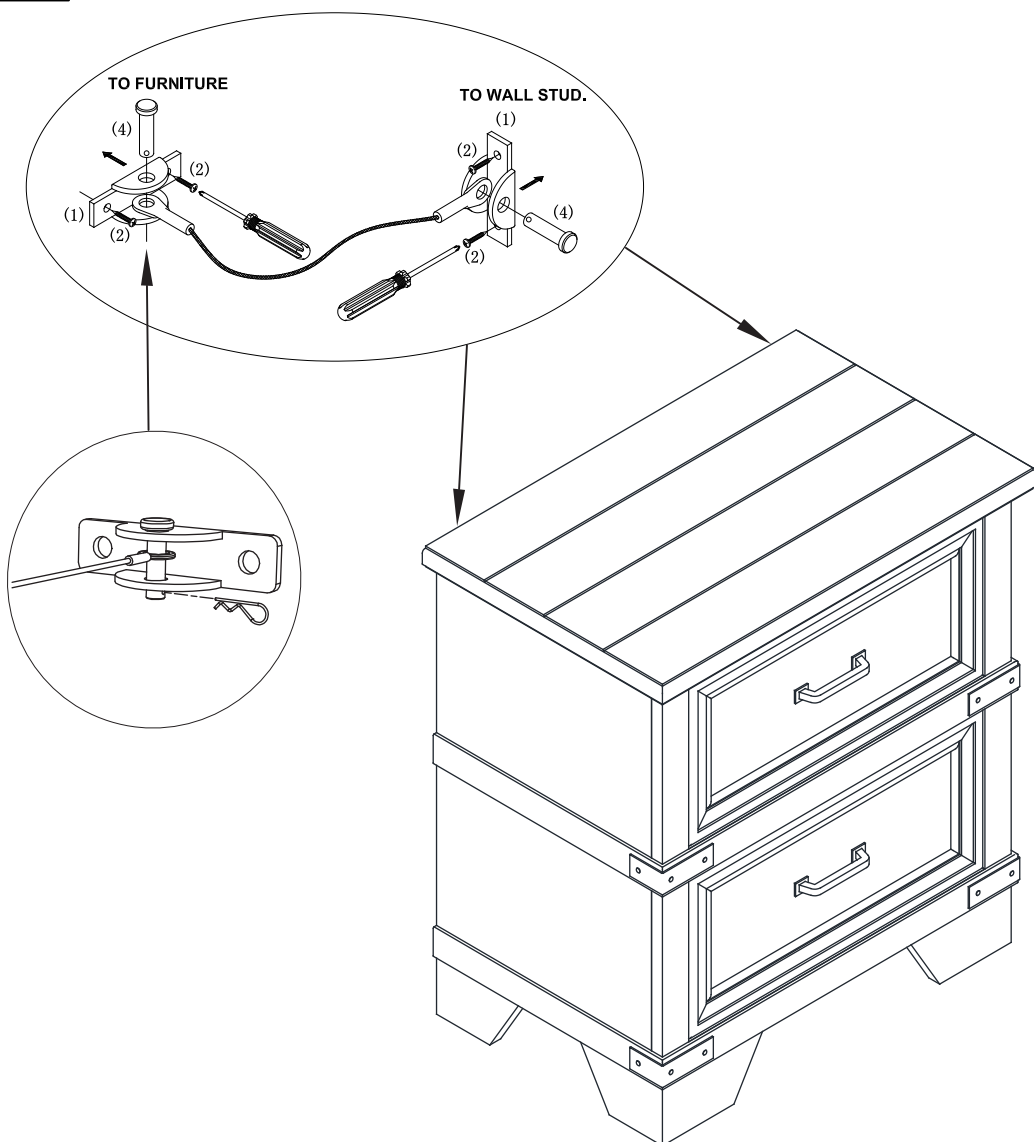
FURNITURE TIPPING RESTRAINT 2 SETS
