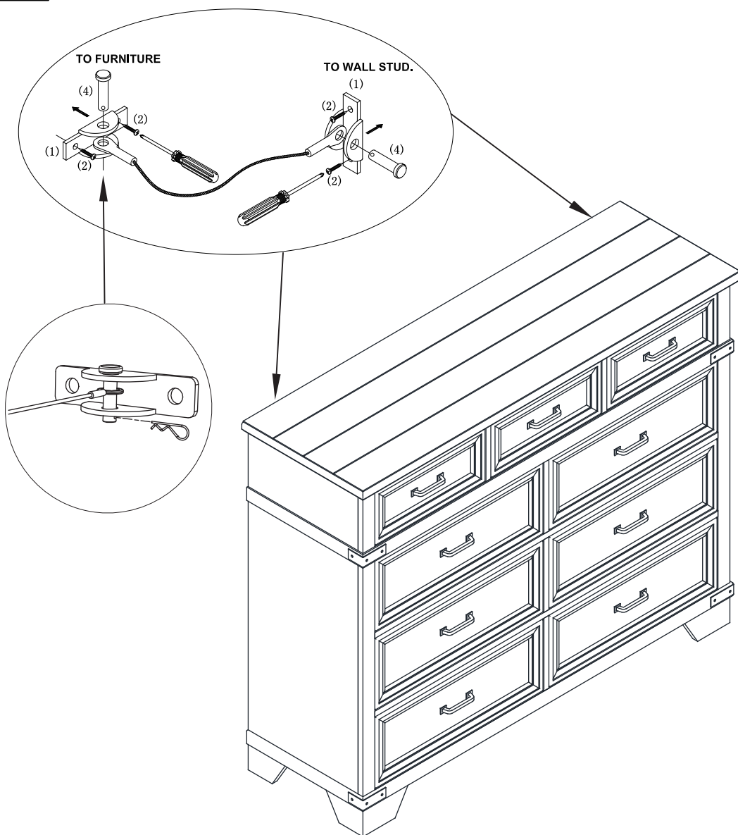
FURNITURE TIPPING RESTRAINT 2 SETS
