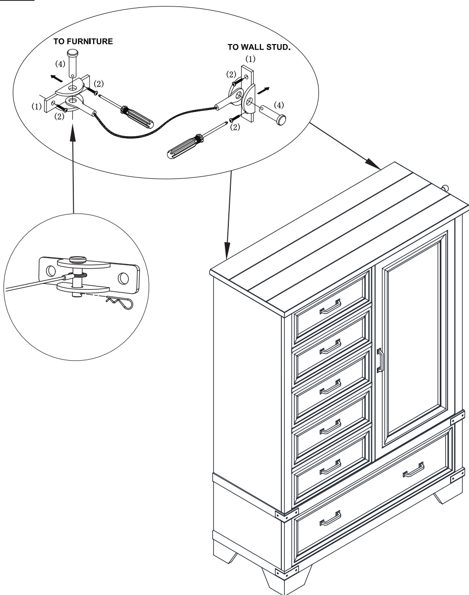
FURNITURE TIPPING RESTRAINT 2 SETS
