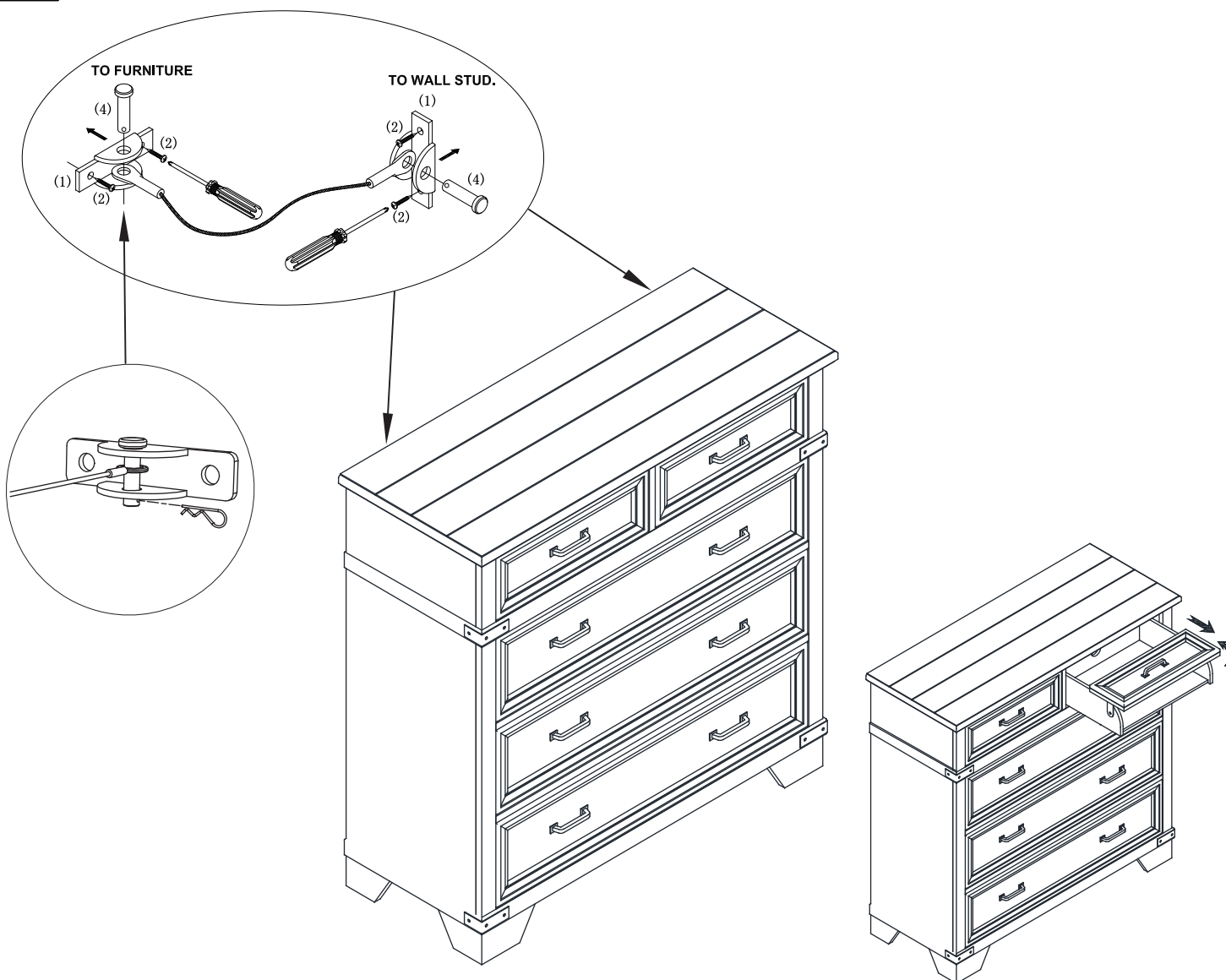
FURNITURE TIPPING RESTRAINT 2 SETS
