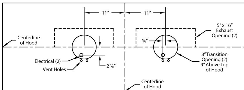
1100 CFM T2+200 Dual Blowers (Top View)
