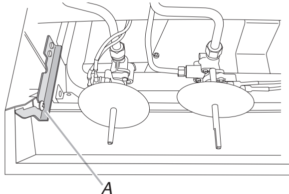
A. Control console bracket
