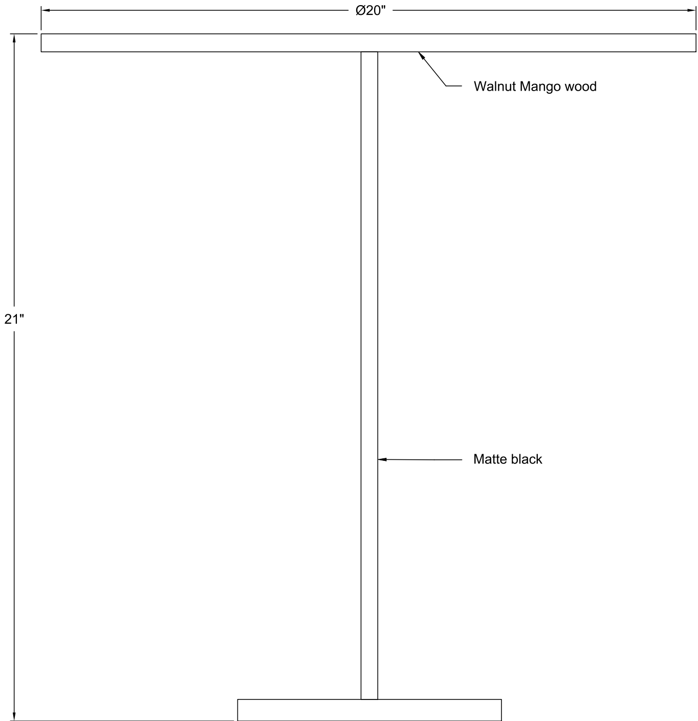
FRONT VIEW
