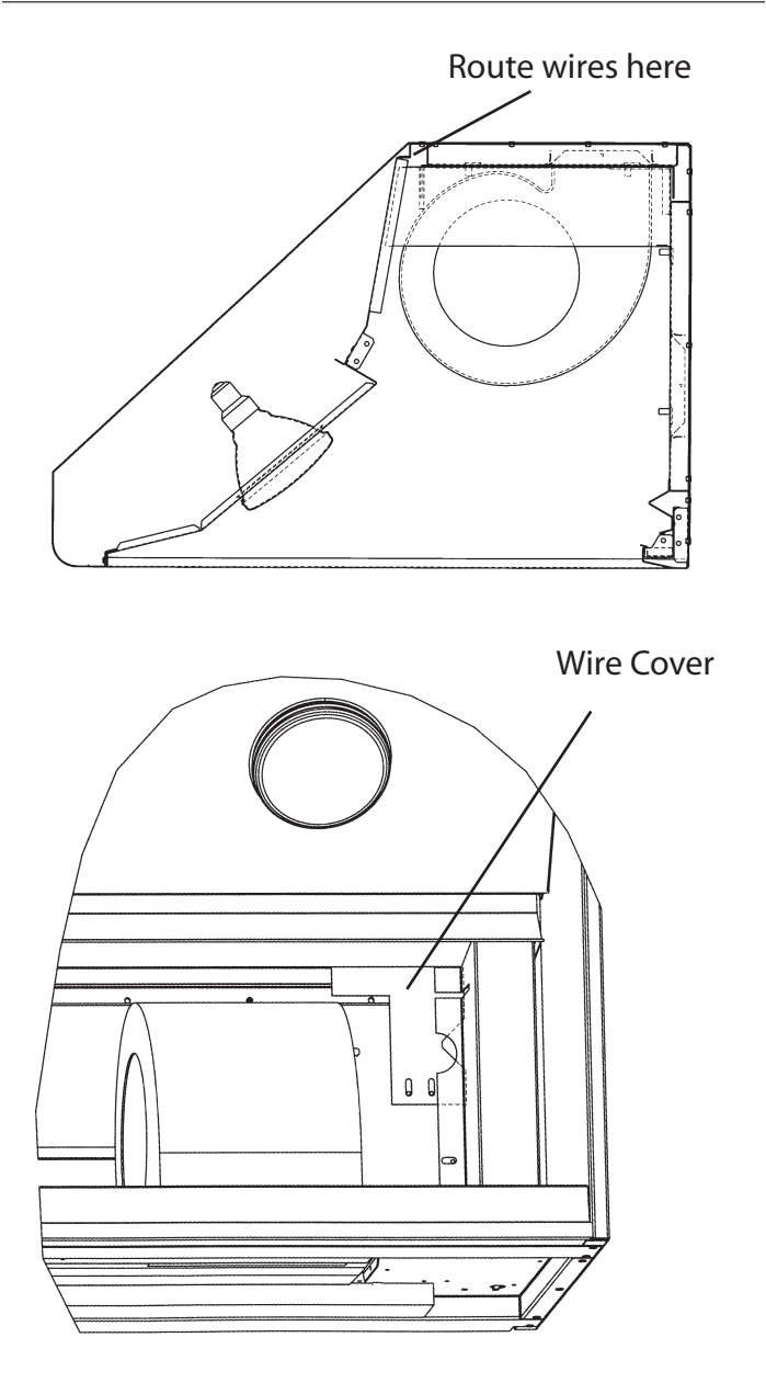
Figure 24: Vertical Discharge
