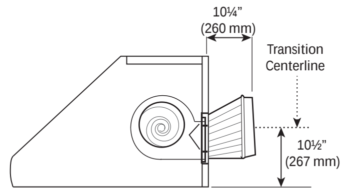
Figure 10: Transition Centerline for Horizontal Discharge
