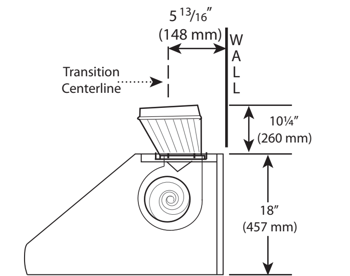
Figure 11: Transition Centerline for Vertical Discharge
