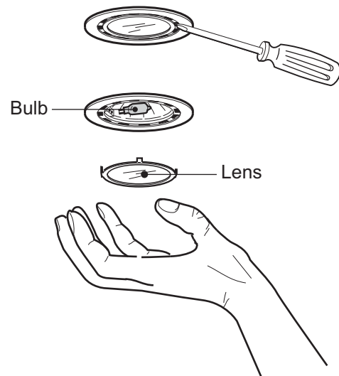
Figure 28: Halogen Light Replacement
