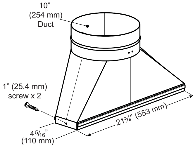
Figure 3: Transition
