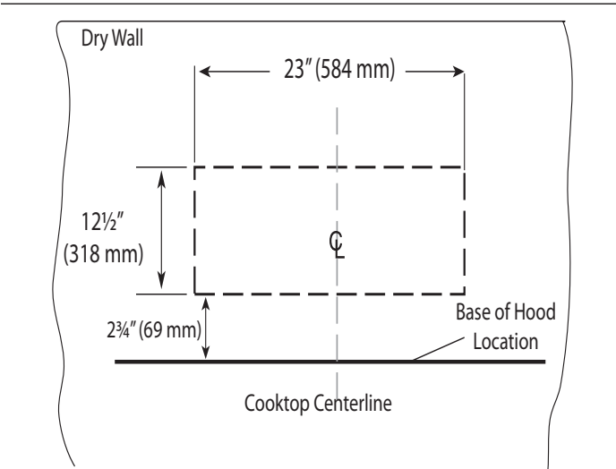
Figure 9: Cutout Dimensions
