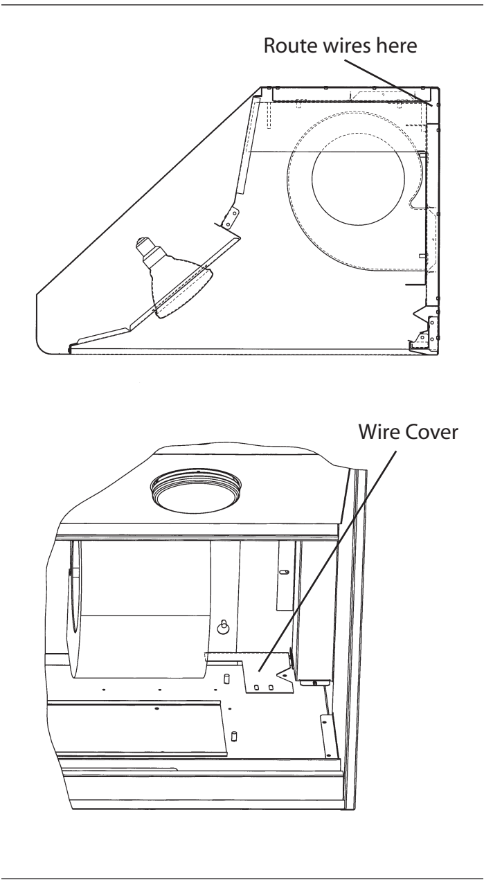
Figure 25: Horizontal Discharge
