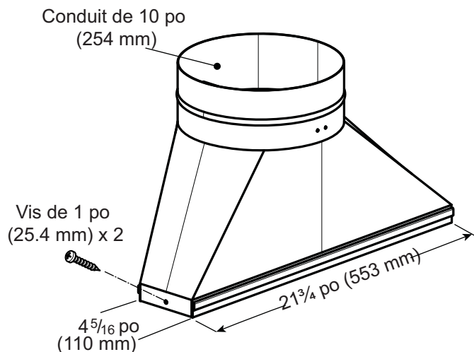
Figure 3 : Raccord
