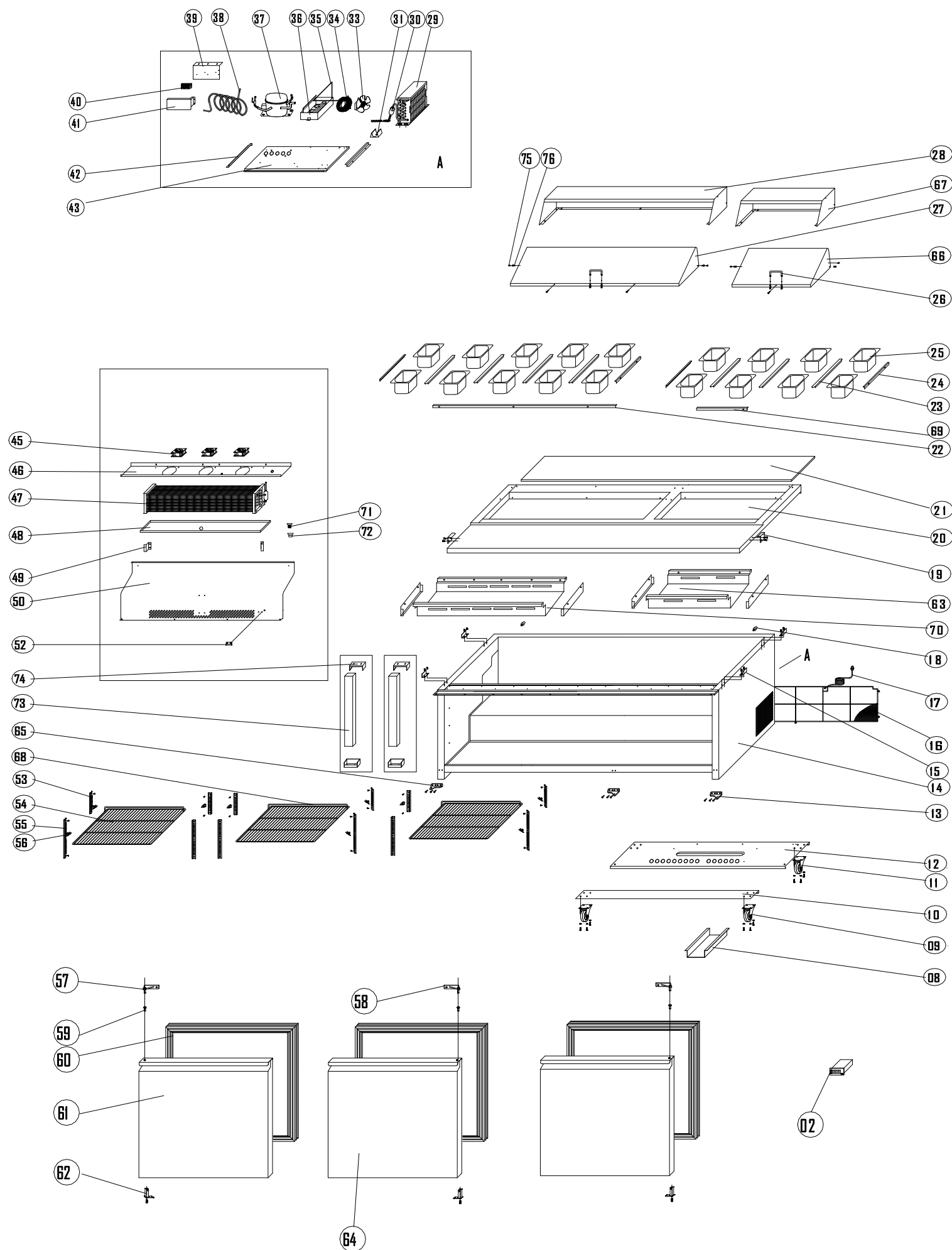
EXPLODE OF KCHST70.18
