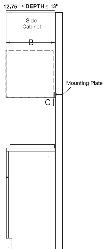
SIDE VIEW
