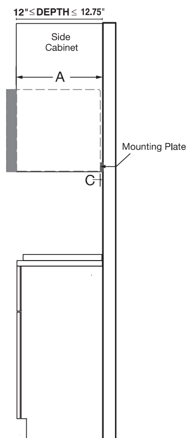
SIDE VIEW
