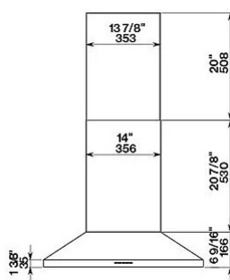
Frontal view
