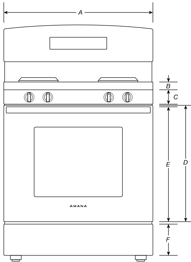
FRONT VIEW
