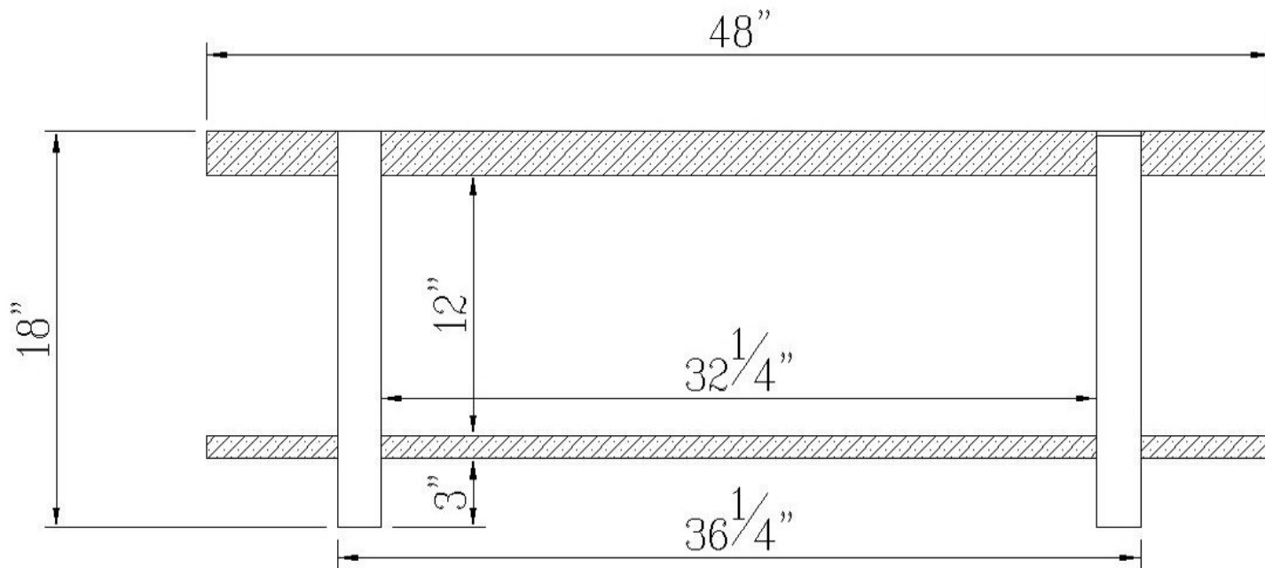
FRONT VIEW
